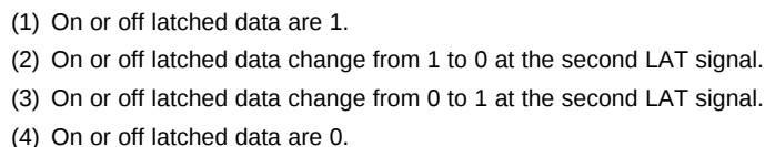
Figure 35. Output On or Off Timing Diagram: Data Write and OUTXn Control
