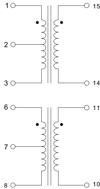
SCHEMATIC "13"
