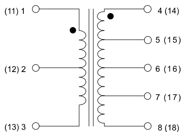
SCHEMATIC "10"
