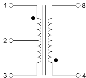
SCHEMATIC "9"
