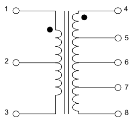
SCHEMATIC "1"
