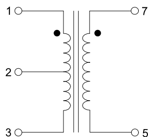
SCHEMATIC "18"
