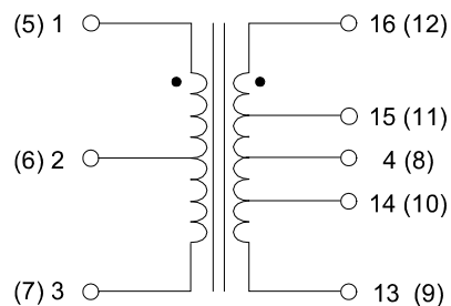
SCHEMATIC "9"
