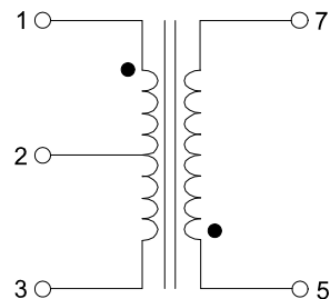
SCHEMATIC "10"
