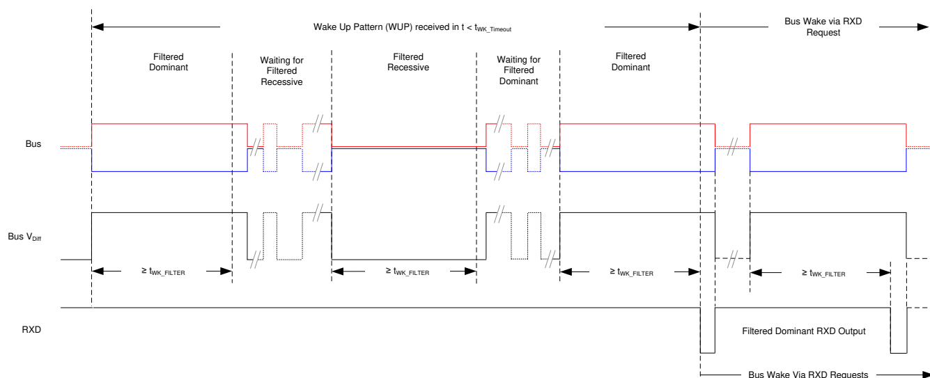
Figure 8-7. Wake-Up Pattern (WUP) with t_{WK\_TIMEOUT}
