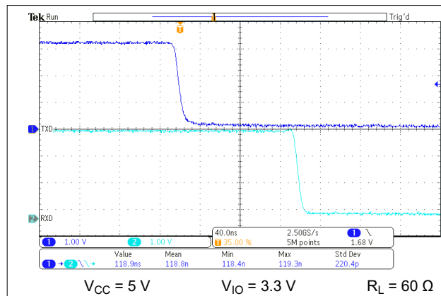
Figure 9-4. t_{\text{PROP(LOOP1)}}
