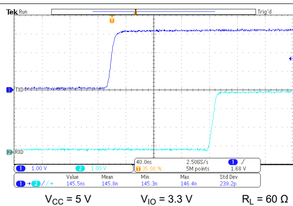
Figure 9-5. t_{\text{PROP(LOOP2)}}
