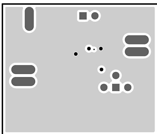
Figure 43. Layer 2 (GND)
