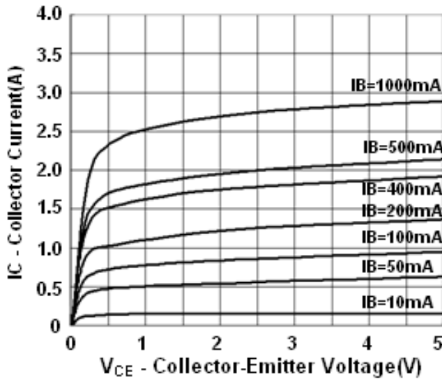
Figure 1. Static Characteristics
