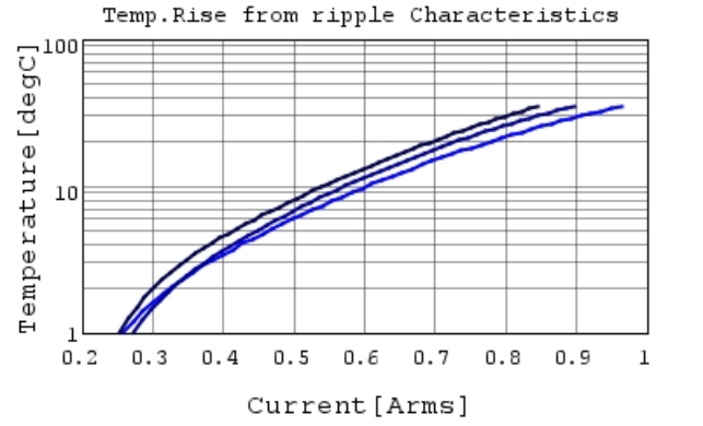
GJM1555C1H6R8CB01 Temp.rise 1GHz 2
