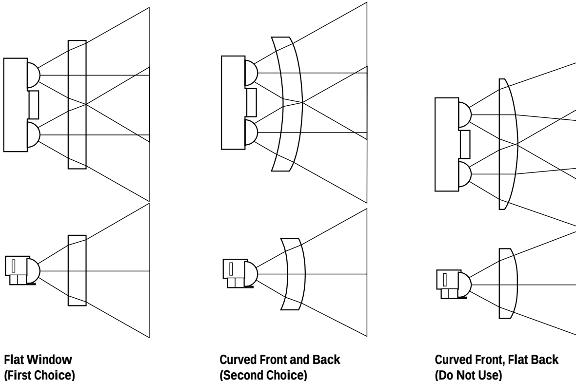
Figure 32. Shape of windows.
