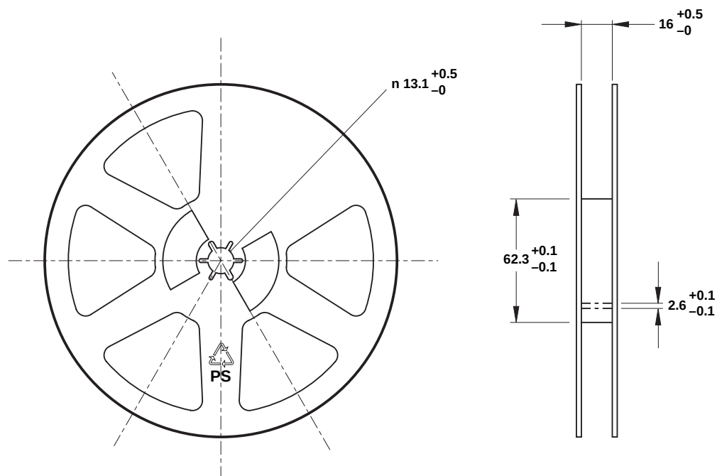
Figure 15. Tape dimensions.
