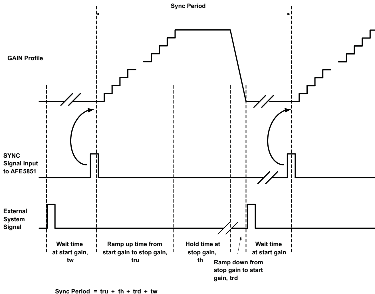
Figure 34. SYNC Period
