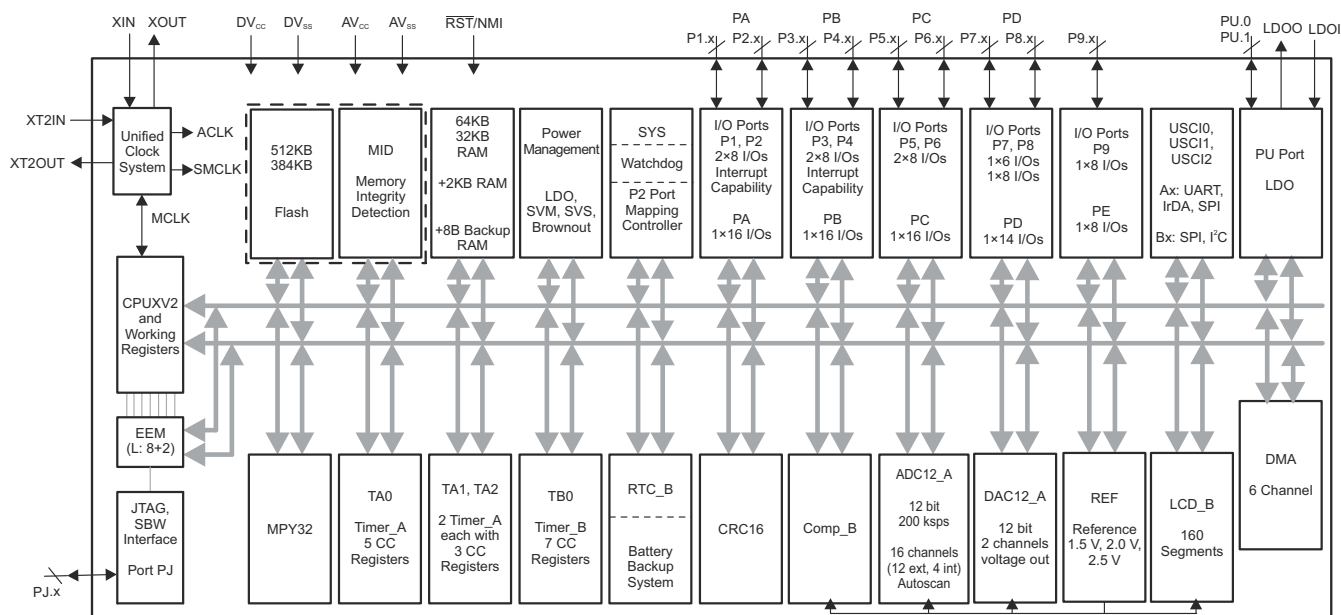
Figure 4-1. Functional Block Diagram – MSP430F6459, MSP430F6458
