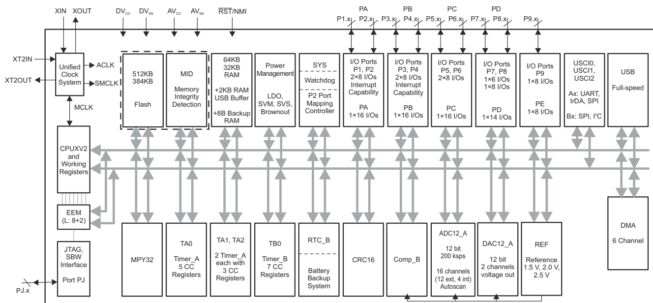
Figure 4-2. Functional Block Diagram – MSP430F5659, MSP430F5658
