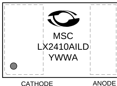
Figure 2 · Pinout DFN 6mmx8mm 2L Top View
