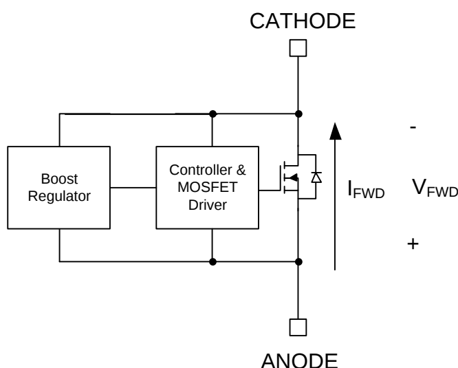
Figure 3 · Simplified Block Diagram of LX2410A
