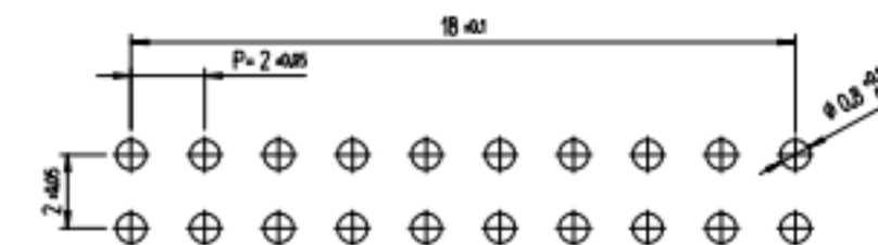
RECOMMENDED LAND PATTERN (FREE) (PCB THICKNESS t=1.6mm)
