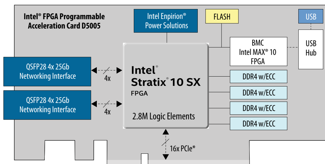
Figure 1. Conceptual Block Diagram
