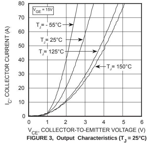
FIGURE 3, Output Characteristics ( T_J = 25^{\circ}\text{C} )
