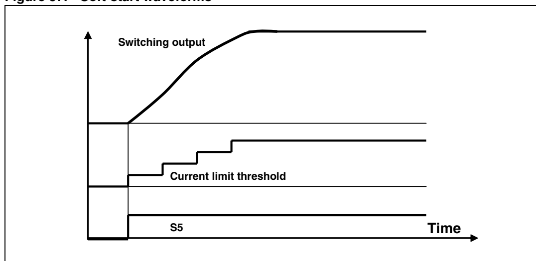
Figure 37. Soft-start waveforms
