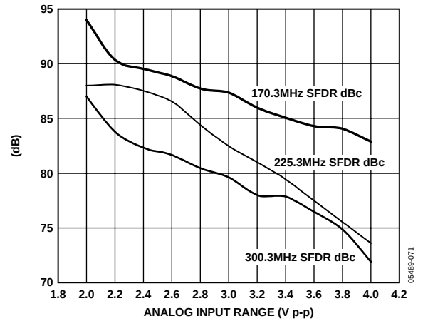
Figure 57. AD9445-105 SFDR vs. Analog Input Range, 105 MSPS/170.3 MHz, 225.3 MHz, 300.3 MHz
