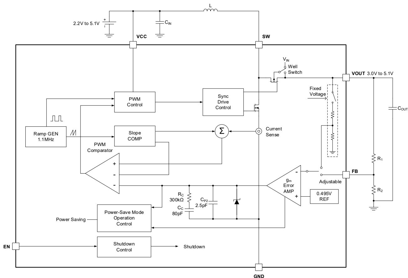
Figure 4. Block Diagram
