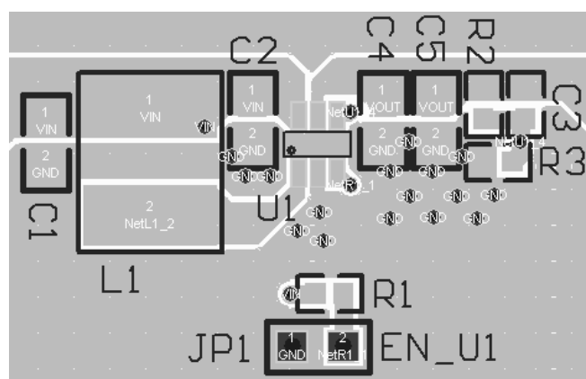
Figure 5. Layout Example
