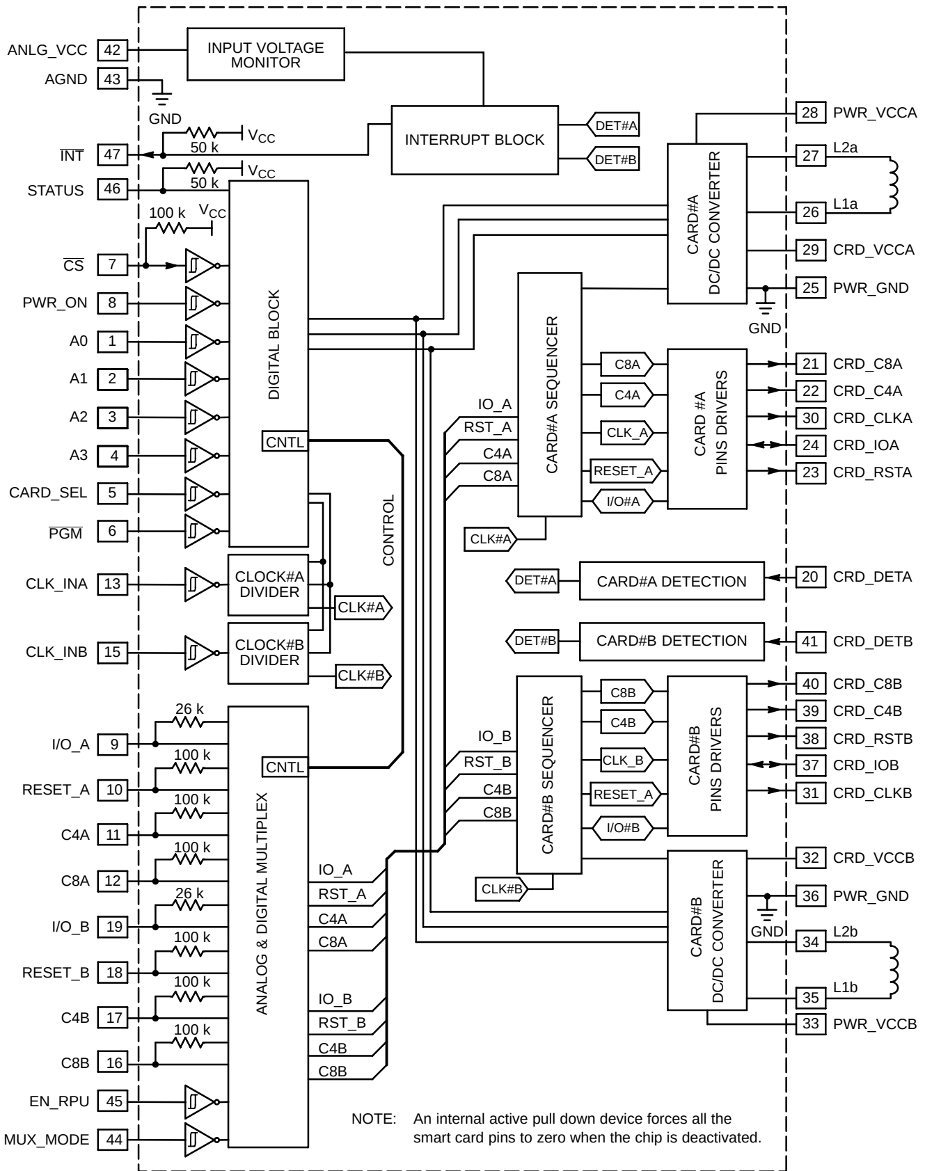
Figure 3. Block Diagram
