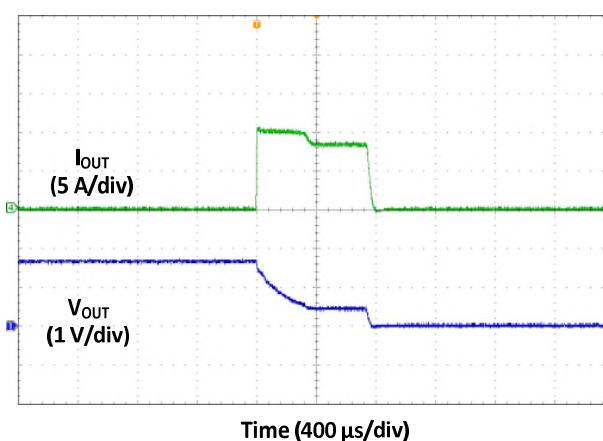
Fig. 37 Hiccup Mode Current Limit Shut-down
