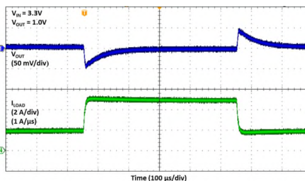
Fig. 17 V_{IN} = 3.3V , V_{OUT} = 1.0V , 3A Load Step
