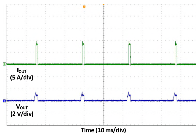
Fig. 39 Hiccup Mode Current Limit Restart into Short-Circuit
