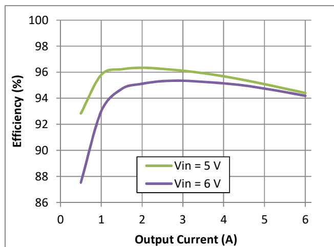
Fig. 1 Efficiency vs Output Current
