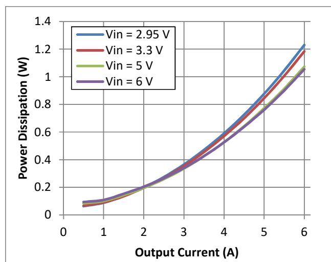
Fig. 12 Power Dissipation vs Output Current
