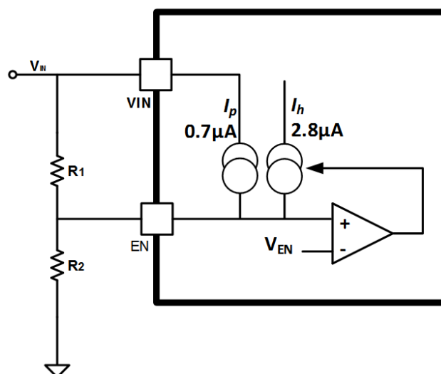
Fig. 28 Input Under-Voltage Lockout Setup
