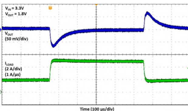
Fig. 21 V_{IN} = 3.3V , V_{OUT} = 1.8V , 3A Load Step
