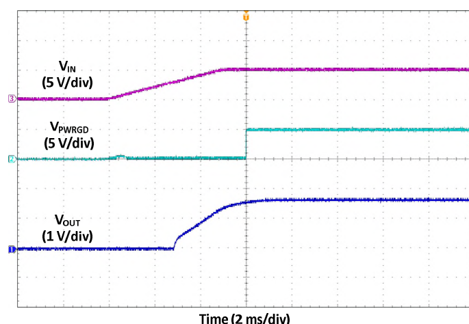
Fig. 24 Startup Waveforms
