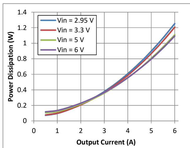
Fig. 10 Power Dissipation vs Output Current
