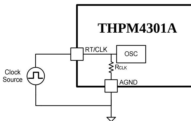
Fig. 35 Synchronizing to a System Clock
