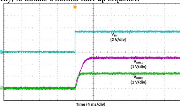
Fig. 32 Tracking Startup, V_{OUT1} = 2.5V , V_{OUT2} = 1.2V
