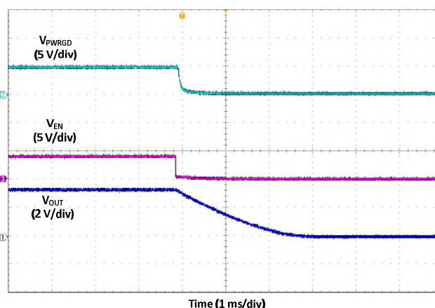
Fig. 27 Waveforms at Enable Turn-Off
