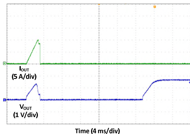
Fig. 38 Recovery from Over-current Shut-down
