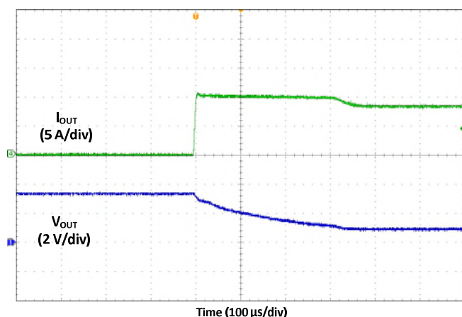
Fig. 36 Over-current Limiting
