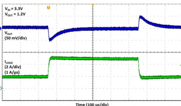
Fig. 19 V_{IN} = 3.3V , V_{OUT} = 1.2V , 3A Load Step
