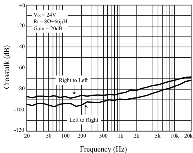
Figure 19 Crosstalk
