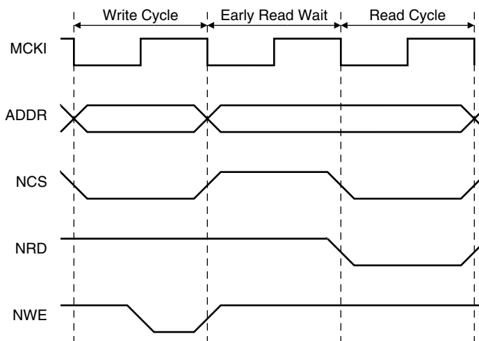
Figure 11-11. Early Read Wait State
