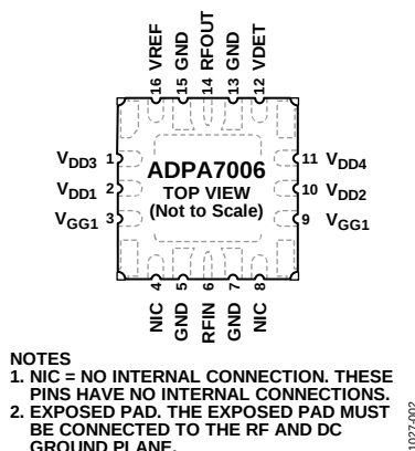
Figure 2. Pin Configuration
