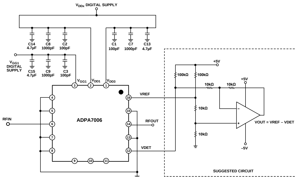
Figure 53. Bias Option 1
