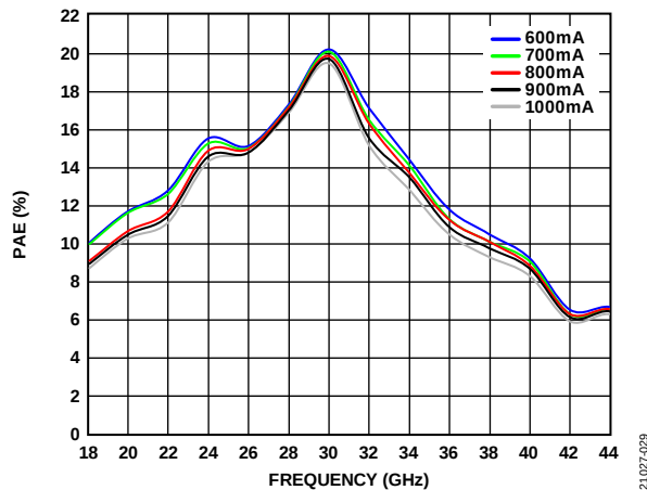
Figure 29. PAE vs. Frequency for Various I_{DQ} , V_{DD} = 5\text{ V} , PAE Measured at P_{SAT}
