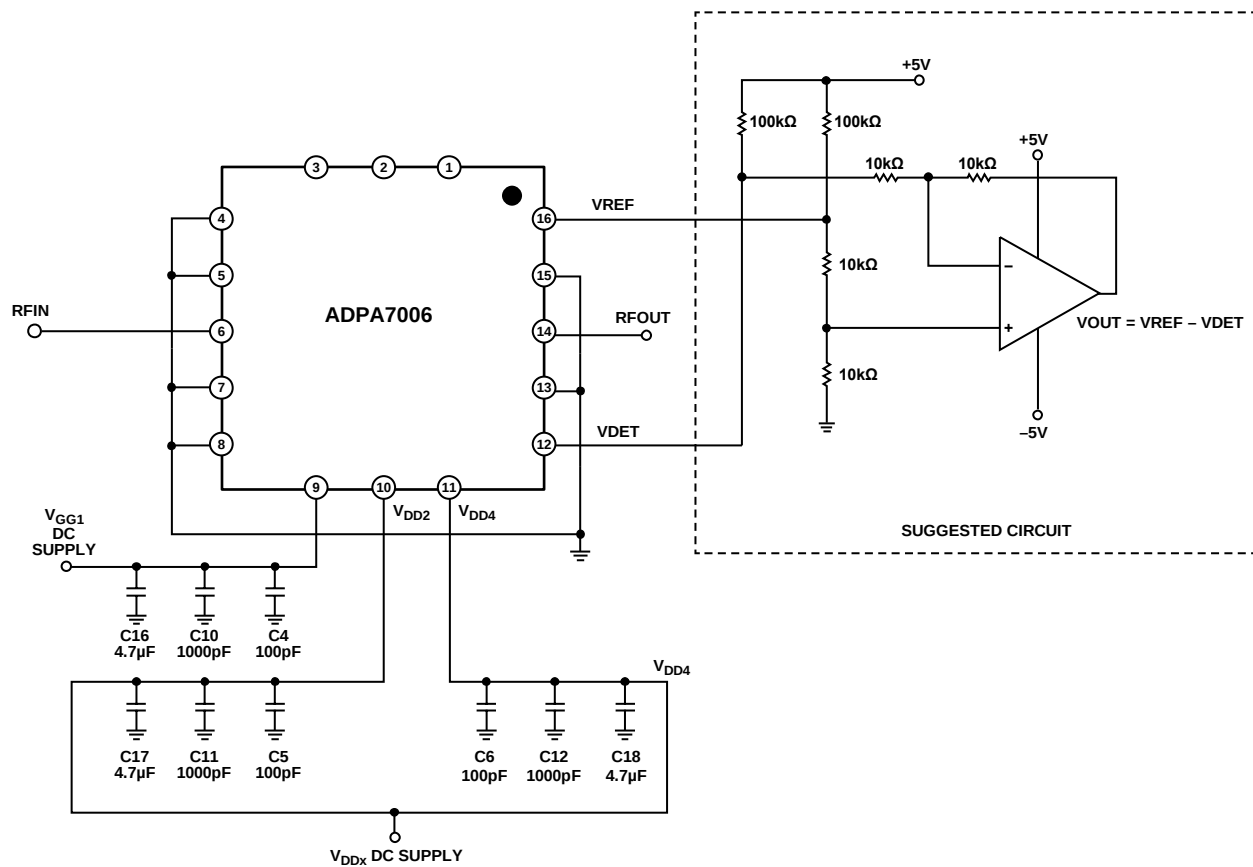
Figure 54. Bias Option 2
