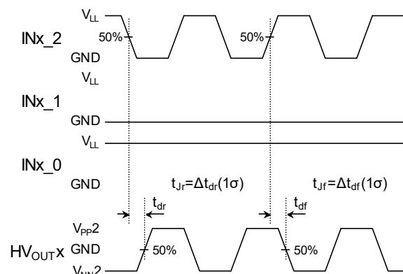
Fig. 7 Delay jitter on rise/fall
