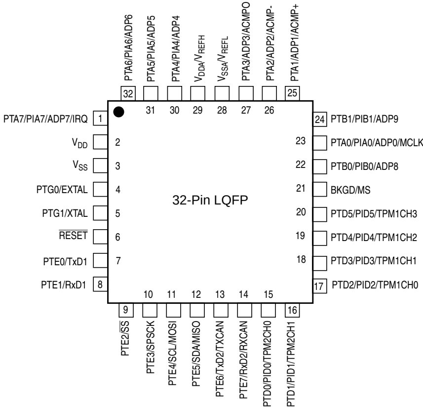
Figure 2-3. 32-Pin LQFP
