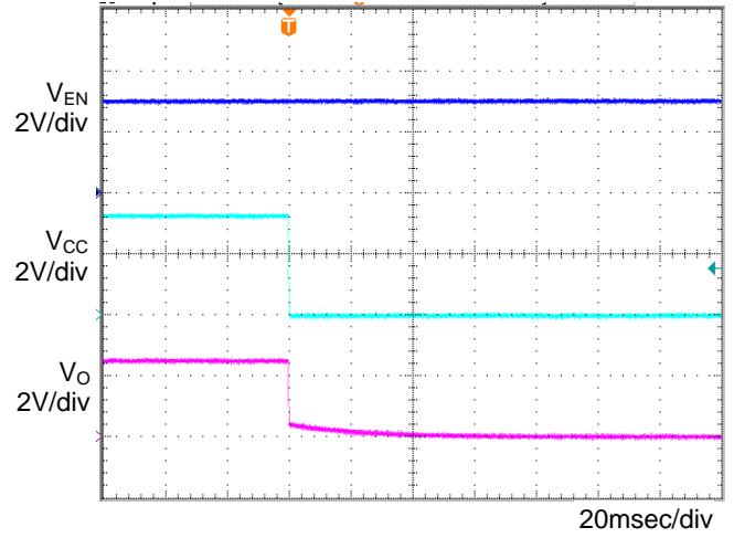
Figure 12. OFF sequence 1 Co=1μF, Ta=-40°C
