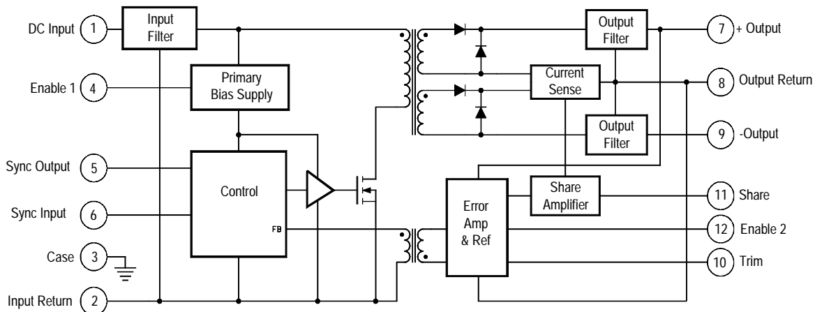
Figure 1. AFL Dual Output Block Diagram
