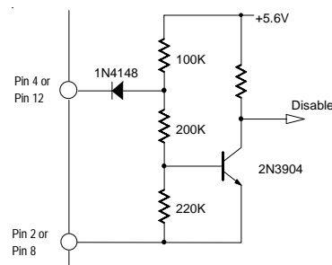
Figure 11. Enable Input Equivalent Circuit
