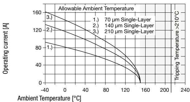
Derating Curve without Shunt (RTS-BC100)
