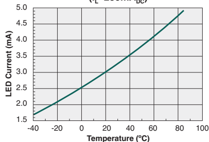
Typical I_F for Switch Operation vs. Temperature ( I_L = 250\text{mA}_{DC} )
