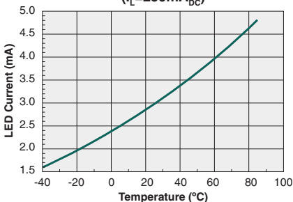
Typical I_F for Switch Dropout vs. Temperature ( I_L = 250\text{mA}_{DC} )
