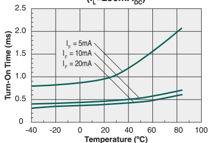
Typical Turn-On Time vs. Temperature ( I_L = 250\text{mA}_{DC} )
