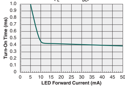
Typical Turn-On Time vs. LED Forward Current ( I_L=250\text{mA}_{DC} )
