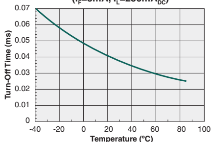
Typical Turn-Off Time vs. Temperature ( I_F = 5\text{mA} , I_L = 250\text{mA}_{DC} )
