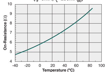
Typical On-Resistance vs. Temperature ( I_F = 5\text{mA} , I_L = 250\text{mA}_{DC} )
