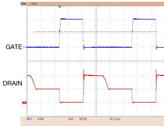
Figure 10. V_{\text{input}} = 48 \text{ V} , I_{\text{out}} = 3.0 \text{ A}
