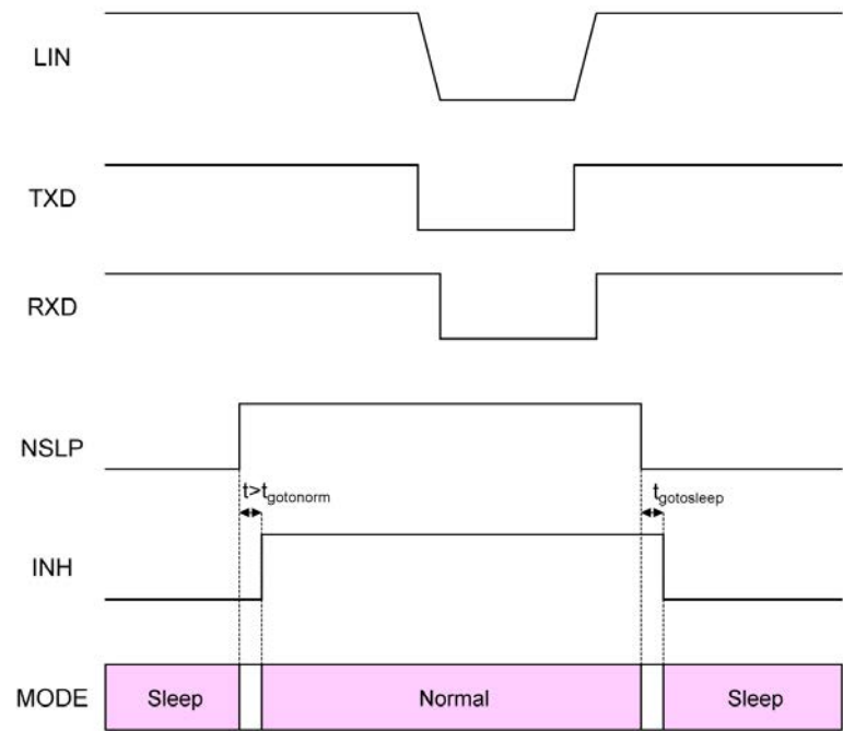
Figure 9. Wake-up/Sleep-in with NSLP (Sleep→Normal→Sleep)
