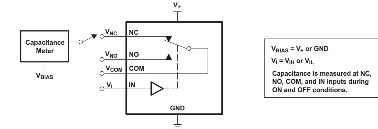
Figure 15. Capacitance ( C_I , C_{COM(ON)} , C_{NC(OFF)} , C_{NO(OFF)} , C_{NC(ON)} , C_{NO(ON)} )
