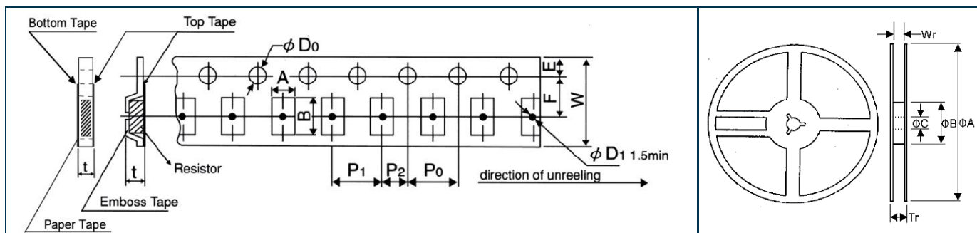
All dimensions in mm
