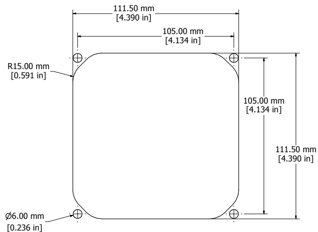
PLATE CUTOUT
