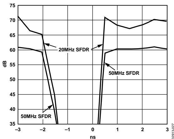
Figure 30. SFDR vs. Clock Placement at f_{OUT} = 20\text{ MHz} and 50\text{ MHz}
