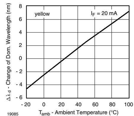
Fig. 24 - Change of Dominant Wavelength vs. Ambient Temperature
