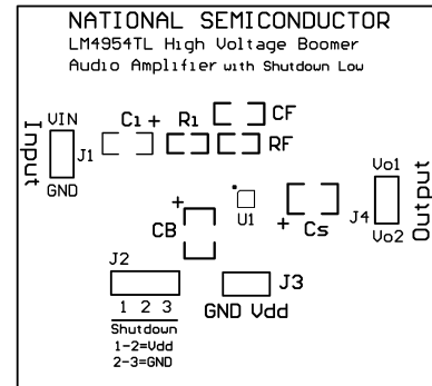
Figure 31. Silk Screen
