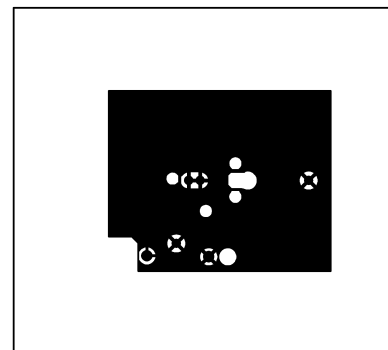
Figure 33. Internal Layer 1, GND
