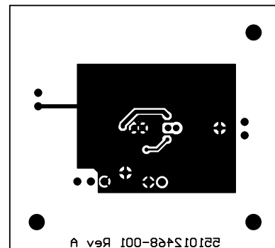
Figure 35. Bottom Layer
