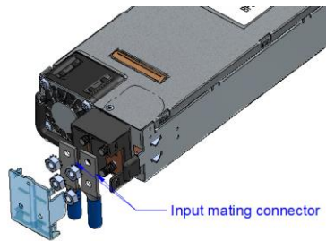
Figure 24. Input mating connector
