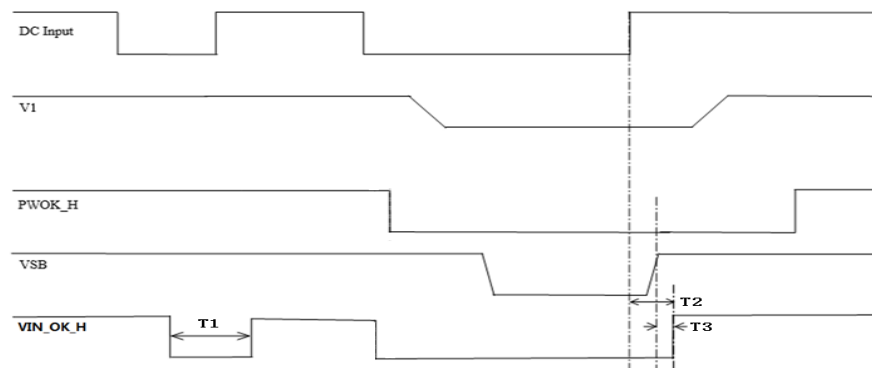
Figure 12. VIN_OK_H Timing
