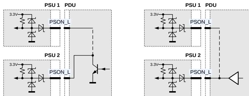
Figure 9. PSON_L connection
