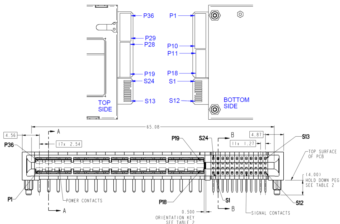
Figure 26. Mating output connector
