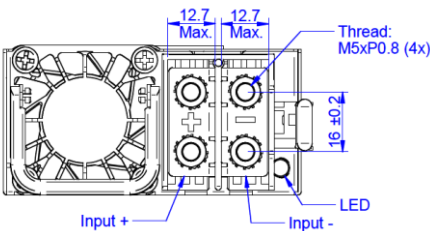
Figure 22. Front view
