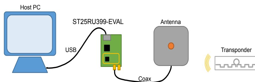
Figure 1. Standard setup
