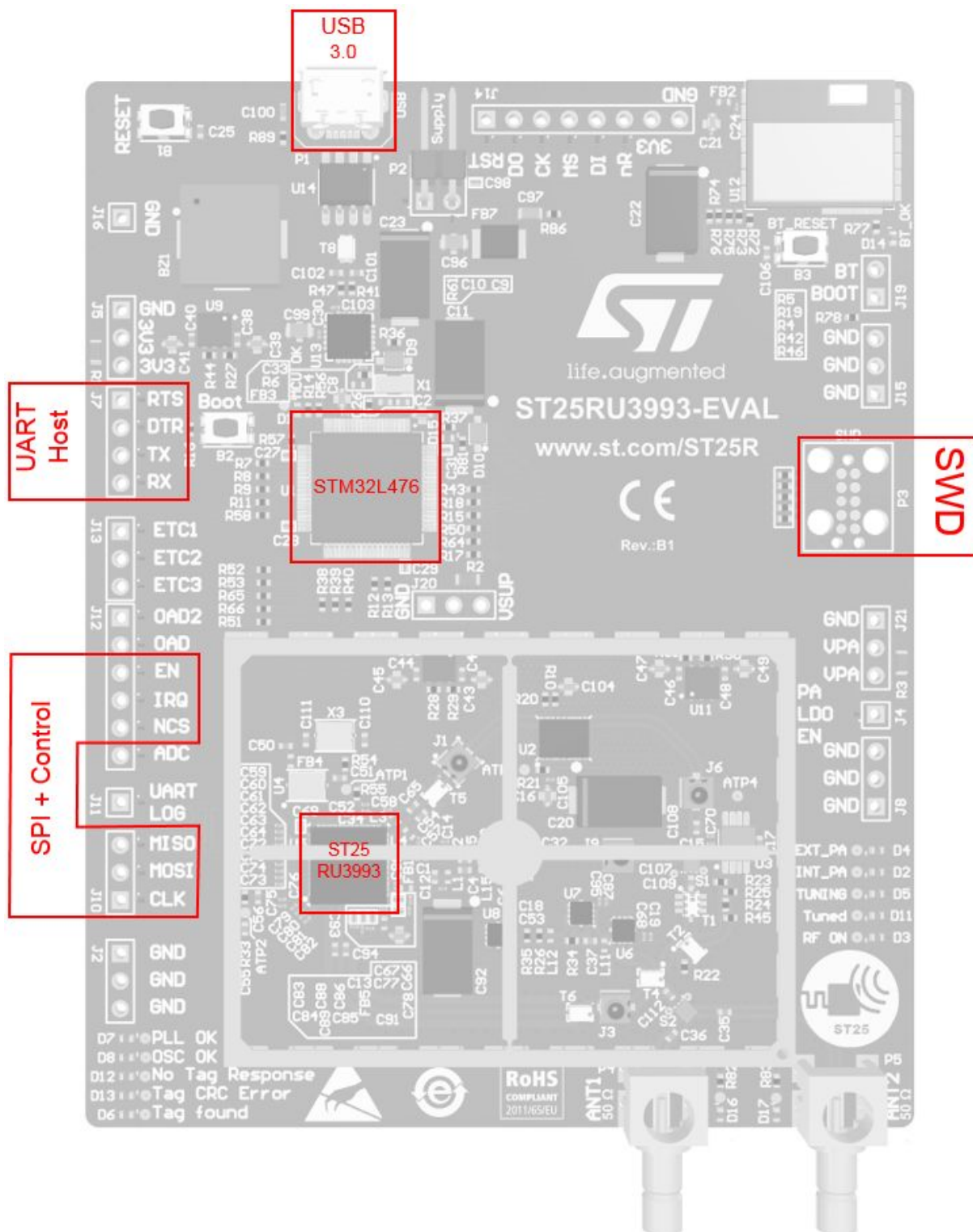
Figure 3. Main digital interfaces and devices on the board
