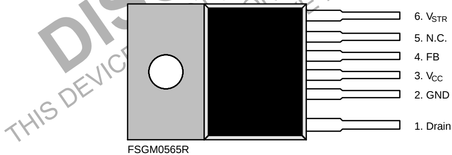
Figure 3. Pin Configuration (Top View)
