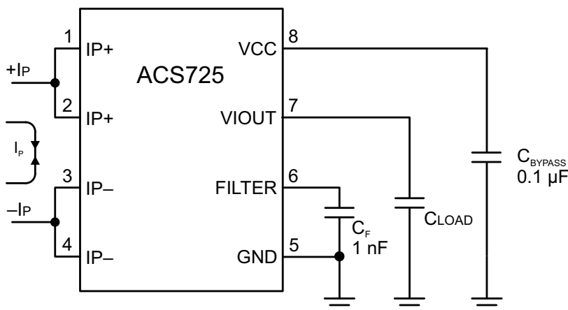
Typical Application
