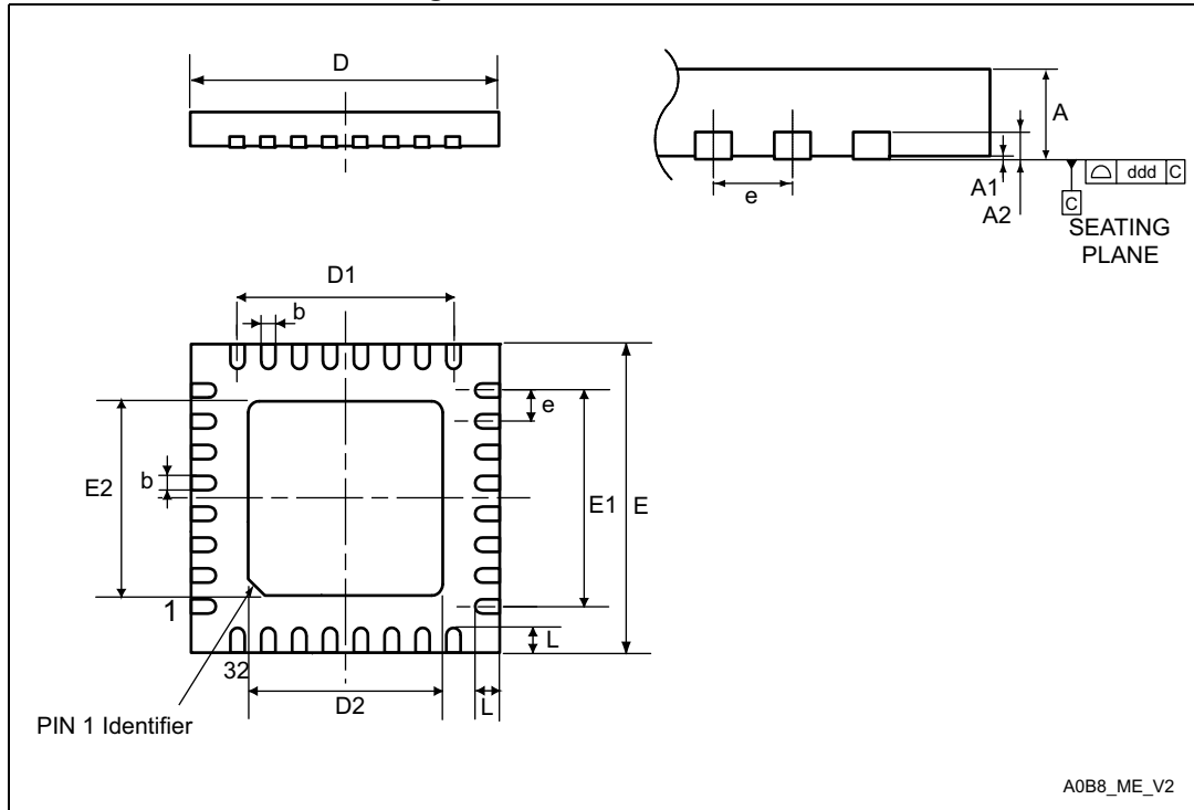
Figure 46. UFQFPN32 outline
