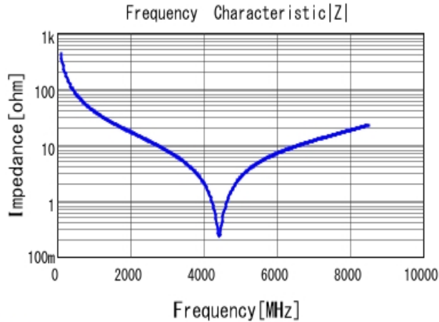
■ GCQ1555C1H3R8WB01 |Z| DC0V, 25degC
