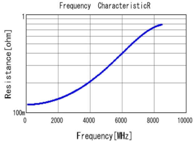
■ GCQ1555C1H3R8WB01 R DC0V, 25degC
