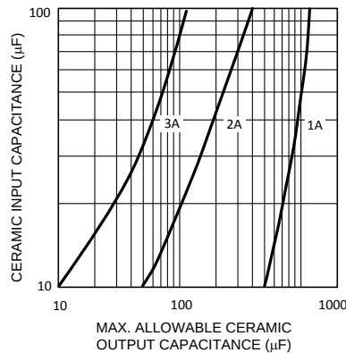
Figure 26. Maximum Ceramic Output Capacitance vs Ceramic Input Capacitance
