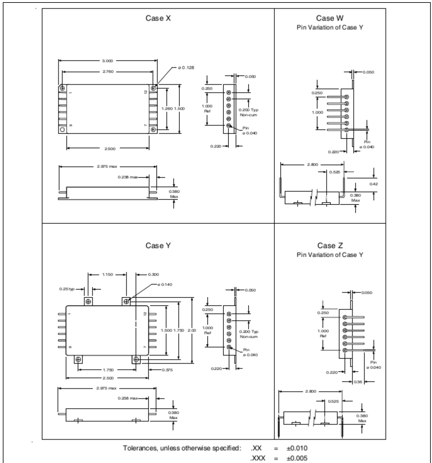
Figure 3 Package outline
