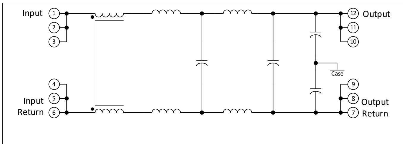
Figure 2 Block Diagram
