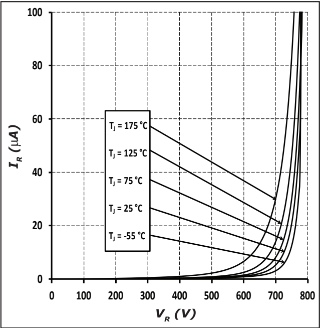
Figure 2. Reverse Characteristics
