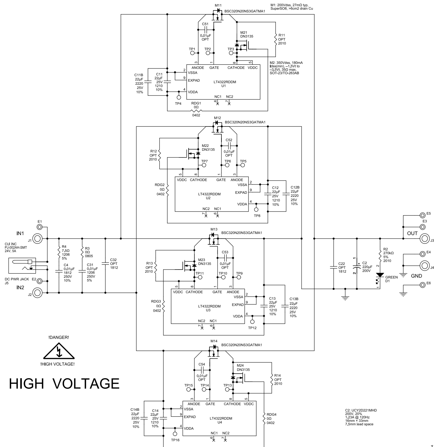
Figure 4. DC3137A Schematic Diagram
