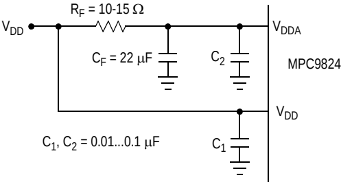
Figure 4. Power Supply Filter
