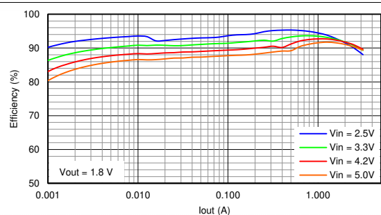
Figure 9-5. Efficiency
