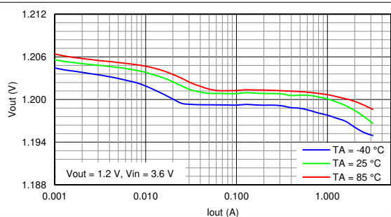
Figure 9-7. Load Regulation
