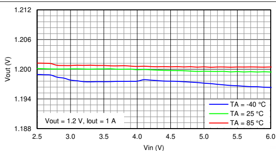
Figure 9-6. Line Regulation
