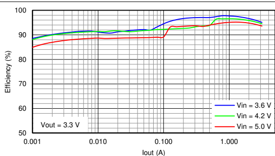
Figure 9-4. Efficiency
