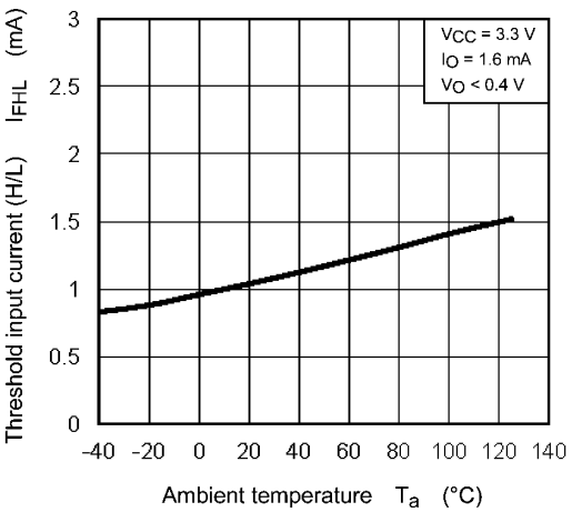
Fig. 12.2.8 I_{FHL} - T_a
