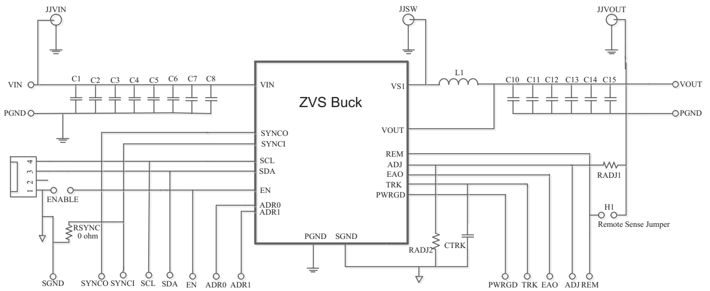
Figure 7 Evaluation board (PCB0190) schematic
