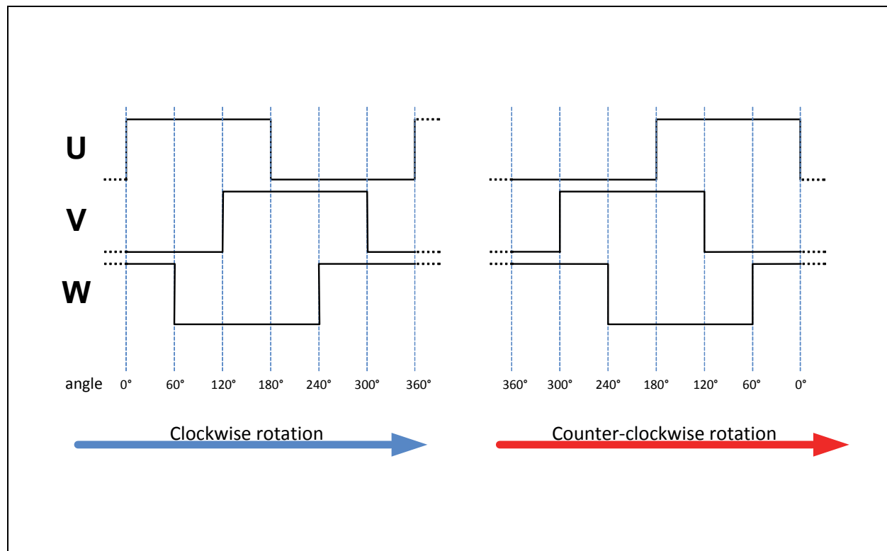
Figure 32: UVW Signals
